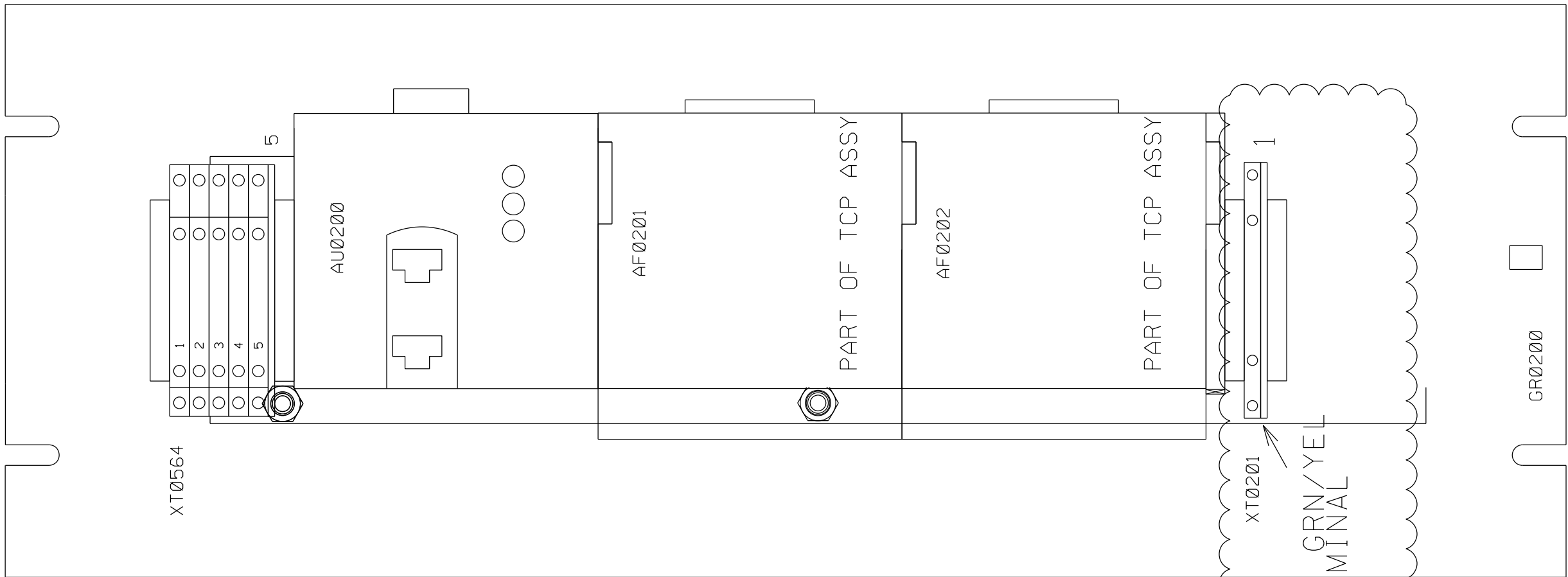
BACK VIEW WITH FLEX I/O INSTALLED
